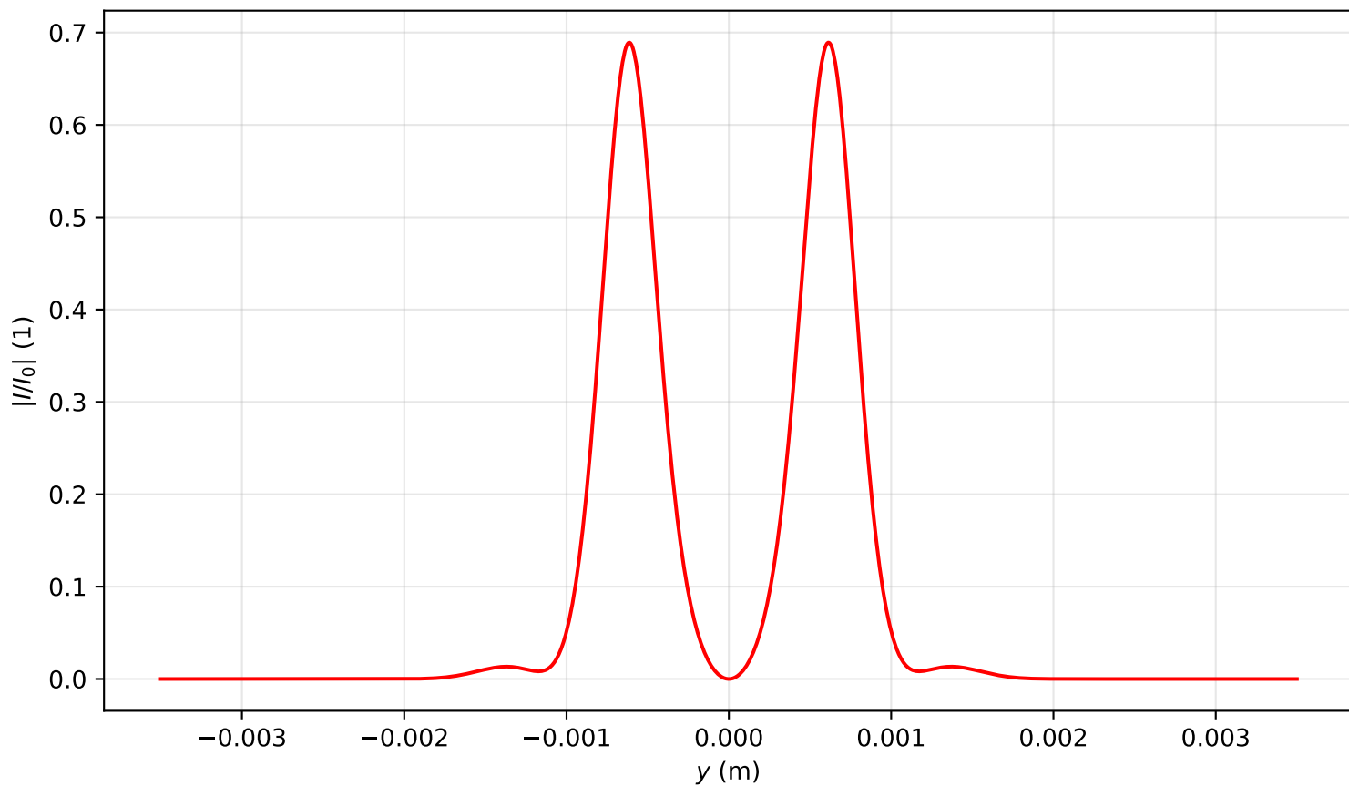
Intensity profile I(x=0, y, z=1.115)/I_0 , \text{Pin}=5.0\text{Pcr} , artificial time
